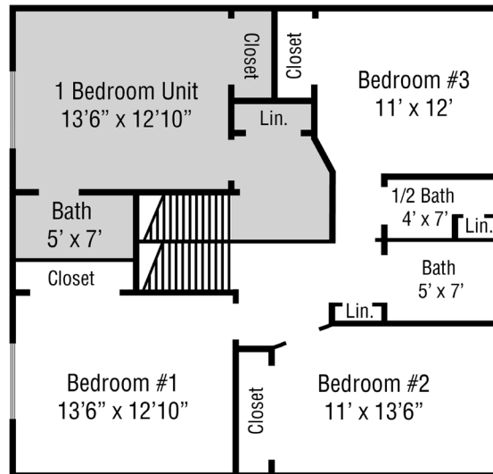
3 & 1 Bedroom combination, 2nd floor Shaded area indicates 1 Bedroom Unit
